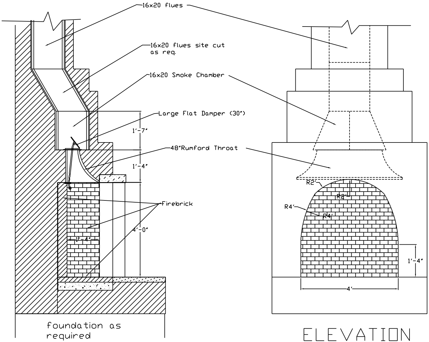
SECTION ELEVATION
