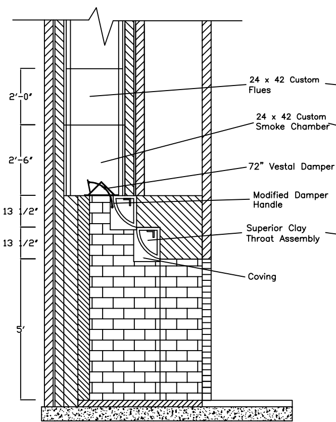
Section Elevation
