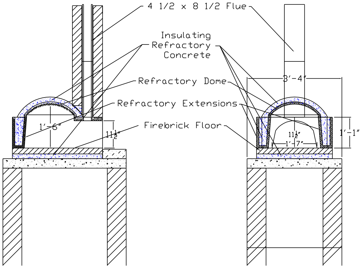
Section A
