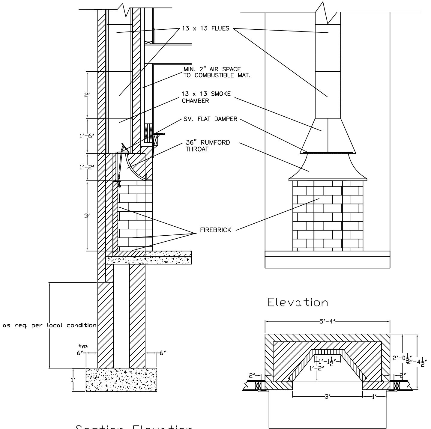
Section-Elevation
