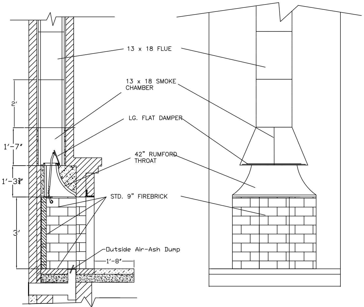
Section – Elevation
