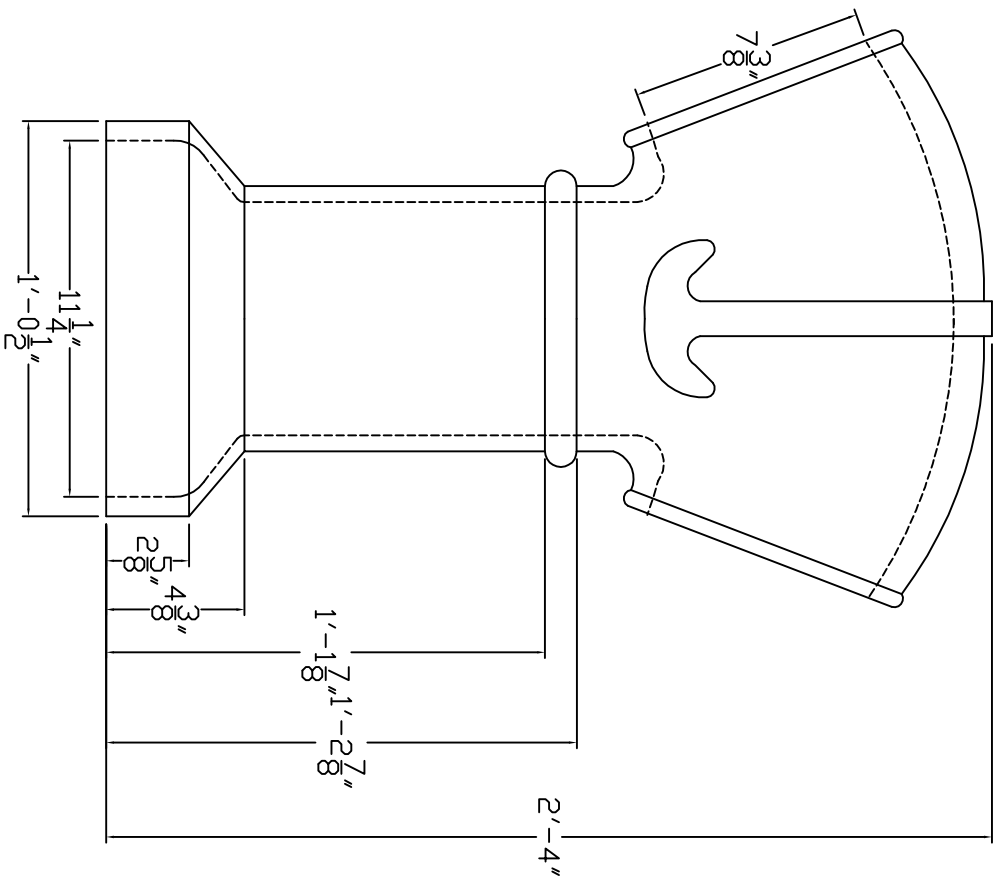
8" Female Anchor Bonnet
