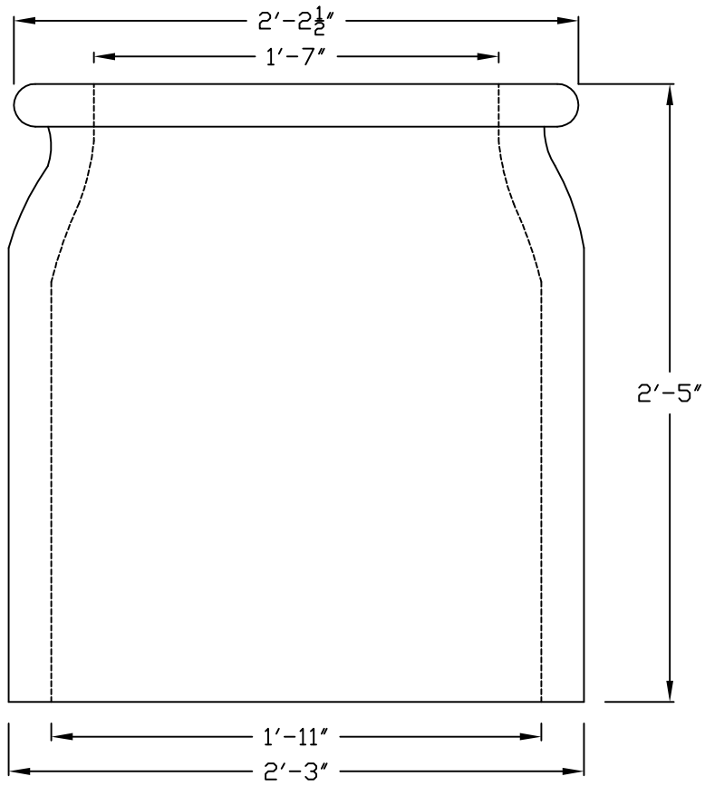
Front View - Archduke Chimney Top
