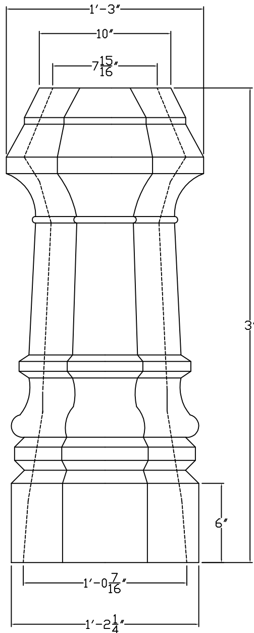
Front View-Austen Top
