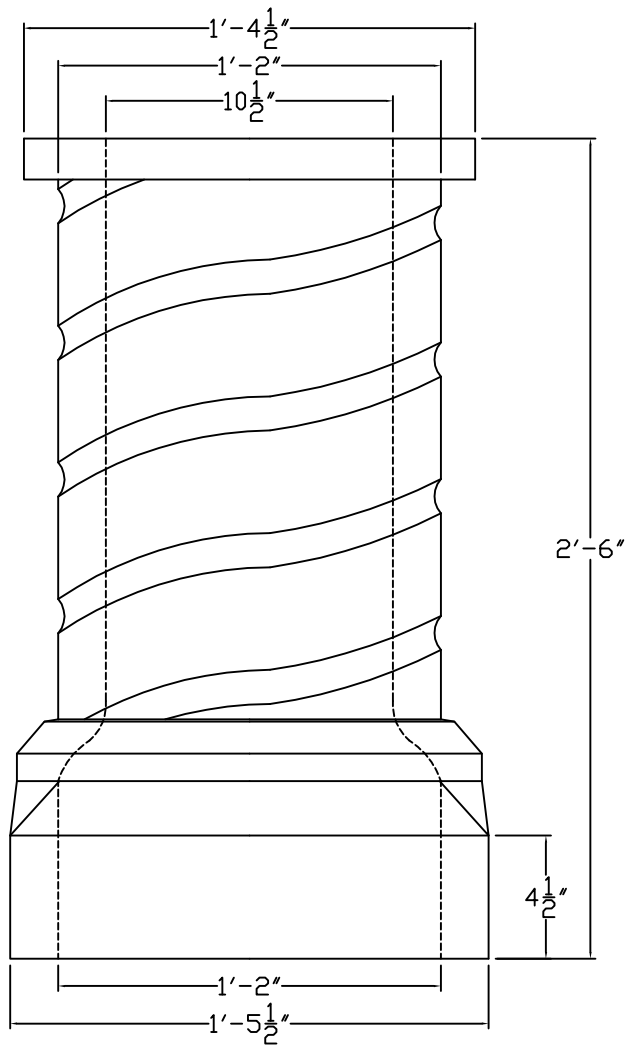
Front View-Top
