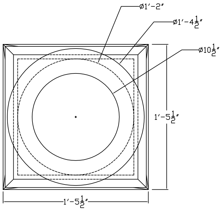
Plan View-Top
