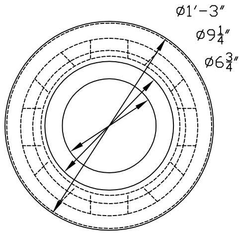
Plan View-Beacon Top
